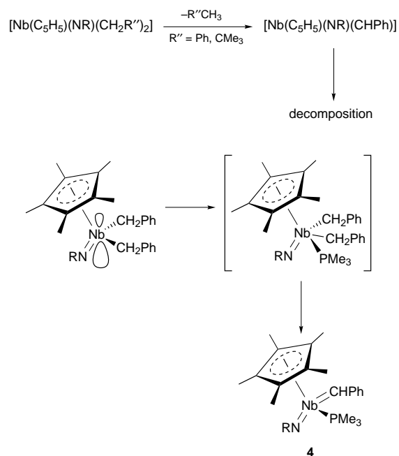
Scheme 7 R = 2,6-Pr t 2 C 6 H 4
